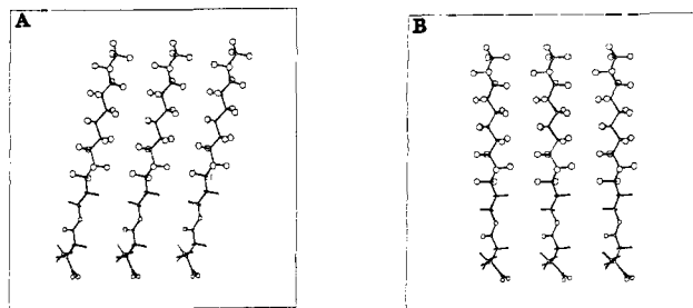
Figure 6. Models for the structure of a Langmuir monolayer of compound 3 . (A) Side view of the \alpha -phase at surface pressures below 25 \text{ dyn/cm} . (B) Side view of the \beta -phase at surface pressures above 25 \text{ dyn/cm} .
