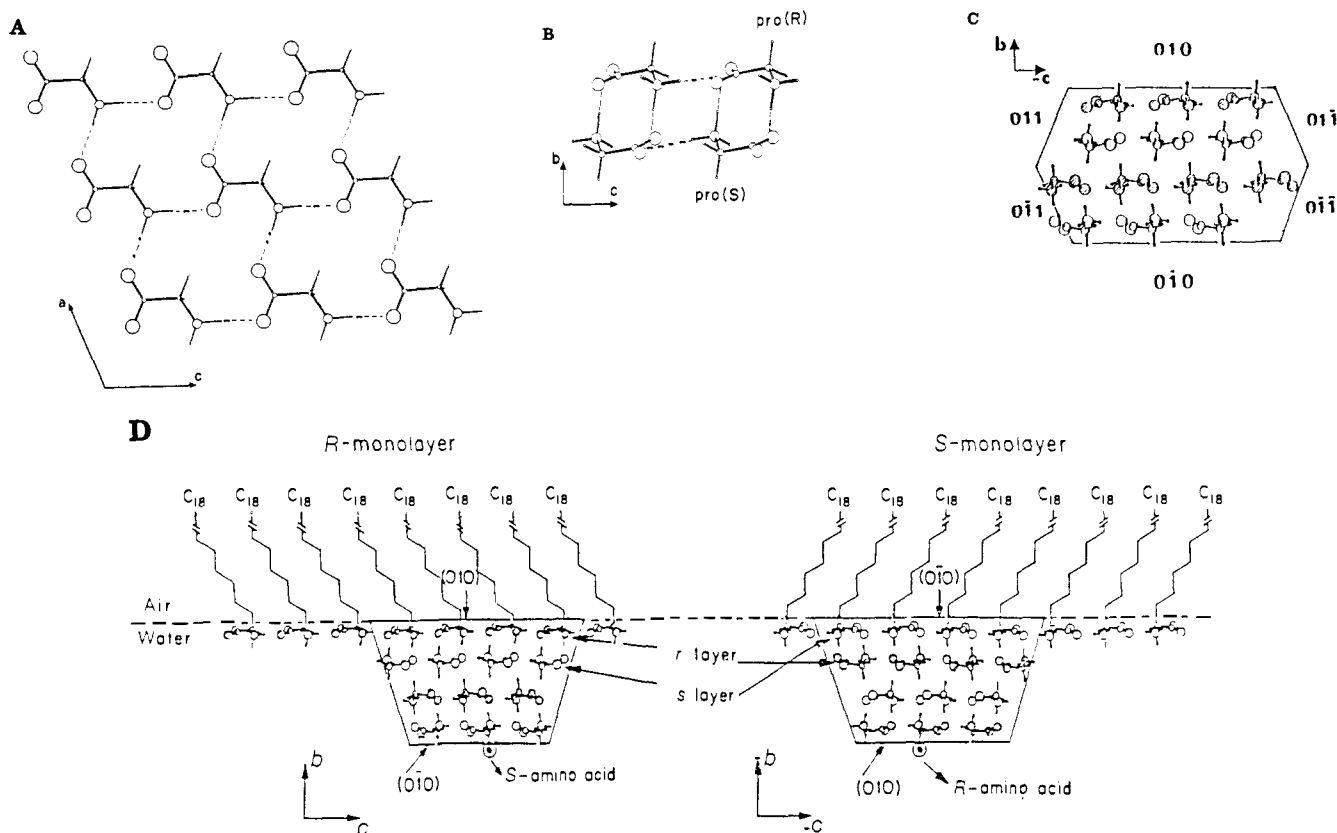
Figure 1. (A) An ac layer of hydrogen-bonded glycine molecules viewed along the b axis. The chiral layer is denoted as r since the H atoms of the C-H bonds that emerge from the ac plane are pro-R . (B) A centrosymmetric bilayer of hydrogen-bonded glycine molecules viewed perpendicular to the bc plane. The upper r layer is that shown in A. (C) Packing arrangement of \alpha -glycine, delineated by its crystal faces. The bilayers (B) are related by 2-fold screw symmetry along the b axis. (D) Schematic views of pyramidal crystals of glycine grown under compressed \alpha -amino acid monolayers of R and S absolute configuration. The (010) face is attached to the R monolayer and the (0 \bar{1} 0) face to the S monolayer. Amino acids of S and R absolute configuration are shown adsorbed from solution at the (0 \bar{1} 0) and (010) faces, respectively.
