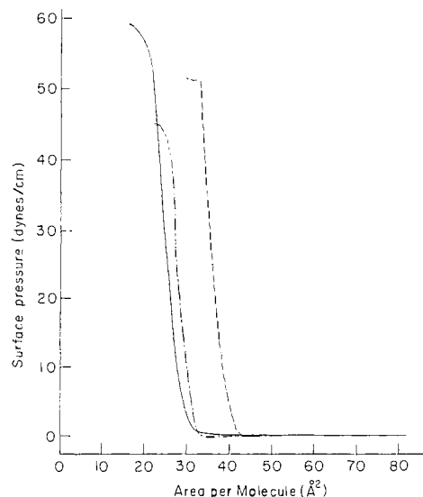
Figure 2. \pi - a diagrams of monolayers 1 (---), 3 (-·-·), and 11 (—) over H 2 O at 20 °C.
