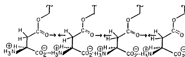
Chart III. Schematic Representation of Compressed Langmuir Monolayers of 11 and 12 : Favorable Interactions between Oxygen Lone Pairs and an Adjacent Methylene
