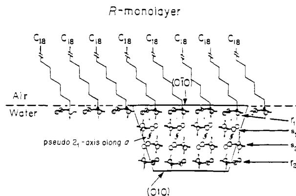
Figure 9. Schematic view of a pyramidal crystal of glycine attached with the (010) crystal face to a compressed R amino acid monolayer.
