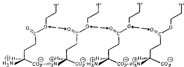
Chart IV. Schematic Representation of a Compressed Langmuir Monolayer of 5 : Repulsion between Oxygen Lone Pairs of Adjacent Molecules
