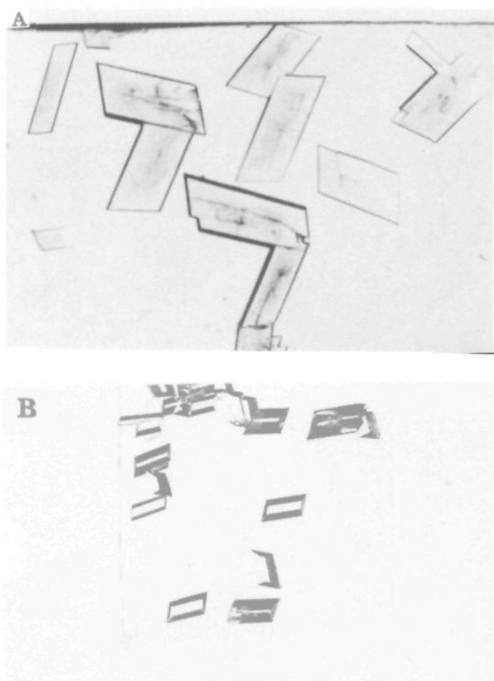
Figure 4. (A) Crystals of glycine grown on a LB film of ( R )- 9 in the presence N ε -(2,4-dinitrophenyl)-( S )-lysine. All the crystals appear as yellow plates attached with their (010) faces to the monolayer. (B) Crystals of glycine grown on a LB film of ( S )- 9 in the presence N ε -(2,4-dinitrophenyl)-( S )-lysine. All the crystals appear as transparent pyramids attached with their (0 \bar{1} 0) faces to the monolayer.
