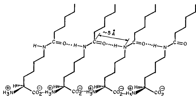
Chart II. Schematic Representation of a Compressed Langmuir Monolayer of 4 : Unfavorable Intermolecular Hydrogen-Bonding Contacts
