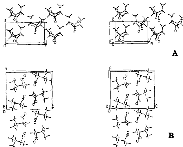
Figure 8. Packing arrangement of crystalline ( S )-valine. 29 (A) Stereoscopic view down the c axis showing the hydrogen-bonded bilayer formed by 2-fold symmetry. There are 2 molecules per asymmetric unit cell, differing in the conformation of the side chains. For clarity, the side chains have been removed. (B) Stereoscopic view down the b axis showing the hydrogen-bonded bilayer formed by 2-fold rotation symmetry.
