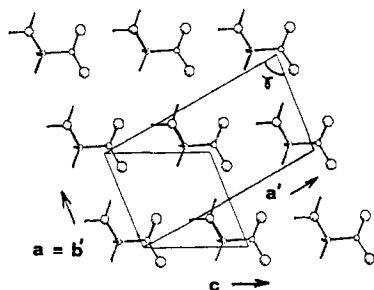
Figure 7. Transformation between the ac lattice of \alpha -glycine and the centered a'b' lattices of the resolved hydrophobic amino acids. The angle between the a and (a + 2c) axes is 87^\circ for \alpha -glycine and 90^\circ for the chiral resolved structures. See also ref 18.
