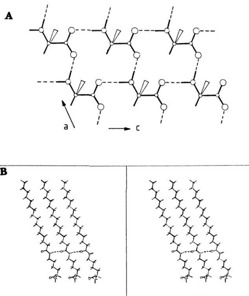
Figure 5. (A) Packing arrangement of palmitoyl-( R )-lysine (compound 9 ) viewed perpendicular to the monolayer. The side chains are represented by wedges. (B) Stereoscopic view along the a - c direction of a row of molecules parallel to the a + c direction. Hydrogen bonding of neighboring secondary amides is denoted by the dashes.
