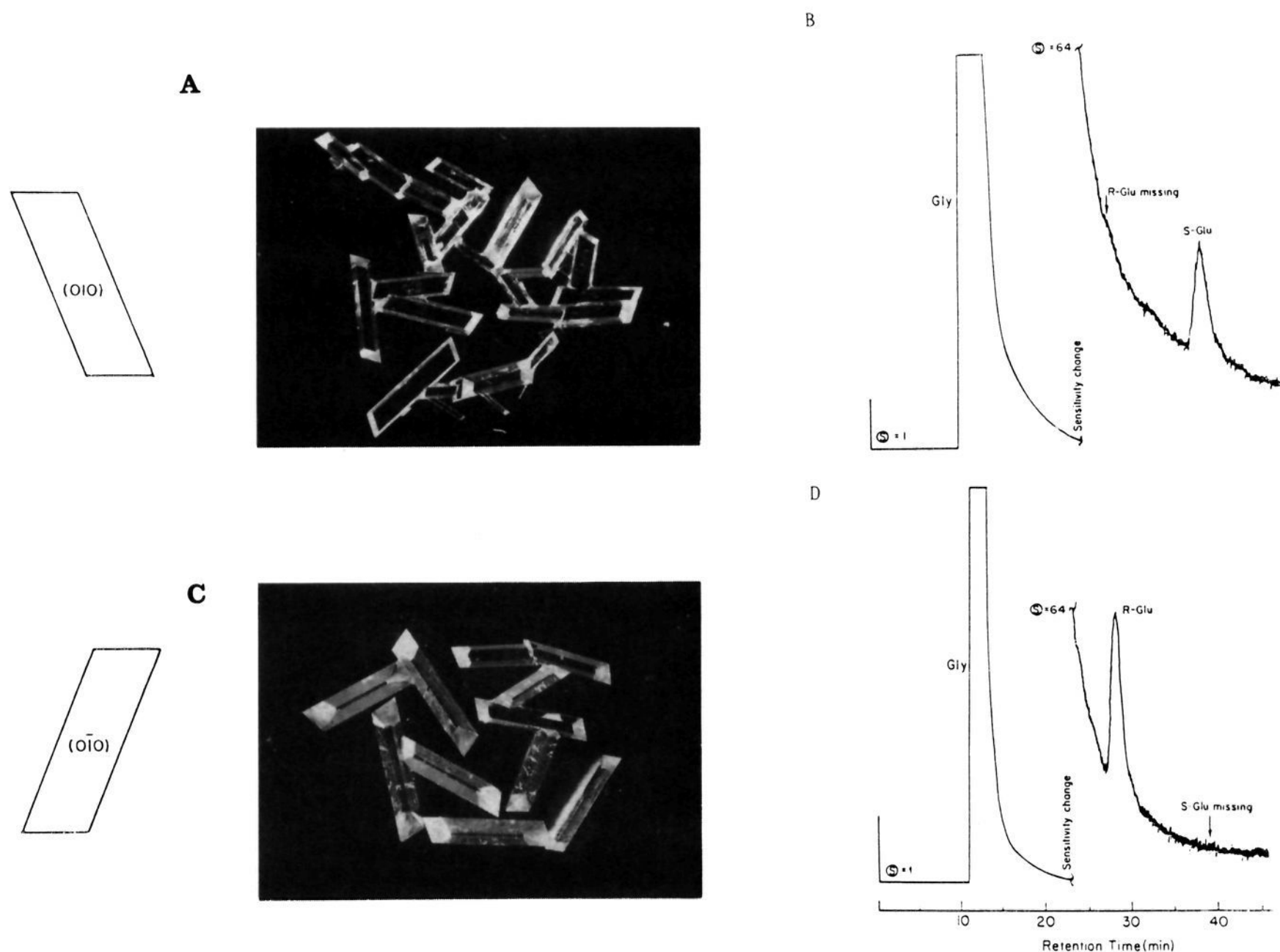
Figure 3. (A) A crust of glycine crystals grown under a monolayer of compound ( R )- 11 in the presence of ( R,S )-Glu. All the crystals are attached with their (010) faces to the monolayer and exhibit the same morphologies. One such crystal is schematically shown as a parallelogram viewed down the b axis. (B) HPLC analysis of an ensemble of crystals grown as in A, after washing with water, sensitivities as indicated. (C) A crust of glycine crystals grown under a monolayer of compound ( S )- 11 in the presence of ( R,S )-Glu. All the crystals are attached with their (0 \bar{1} 0) faces to the monolayer and exhibit enantiomorphous morphologies to those in A. One such crystal is schematically shown as a parallelogram viewed down the -b axis. Note that it is not superimposable on the one depicted in A by rotation in the plane of the air-water interface. (D) HPLC analysis of an ensemble of crystals grown as in C, after washing with water, sensitivities as indicated.
